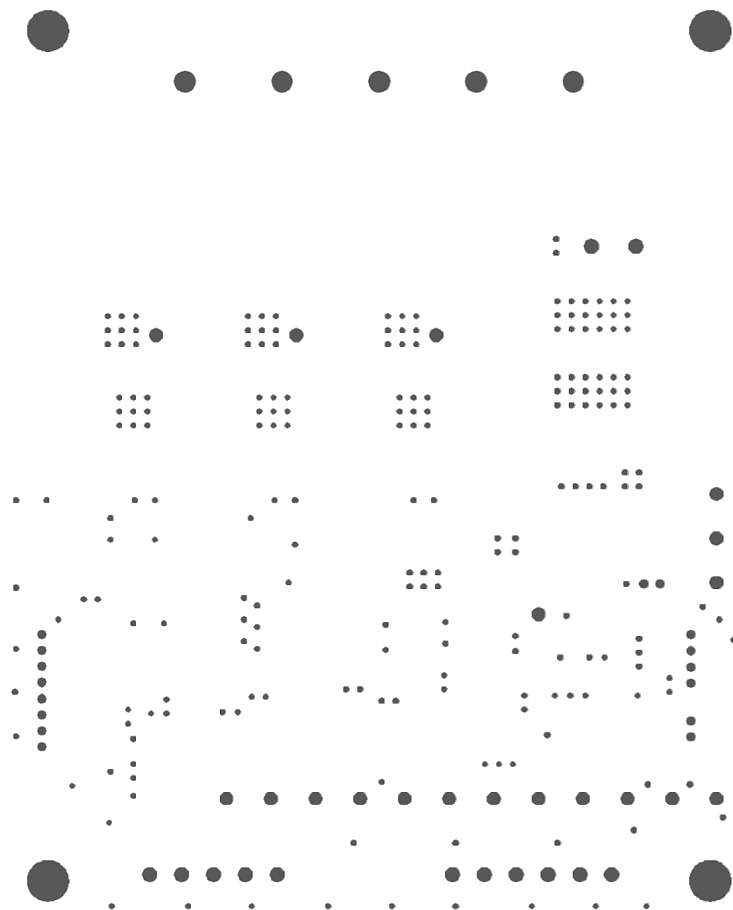
Drill_PTH
