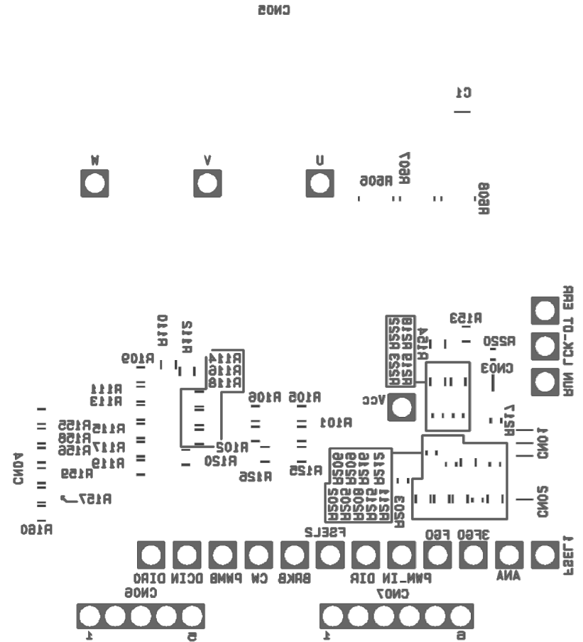
Bottom_Silk
