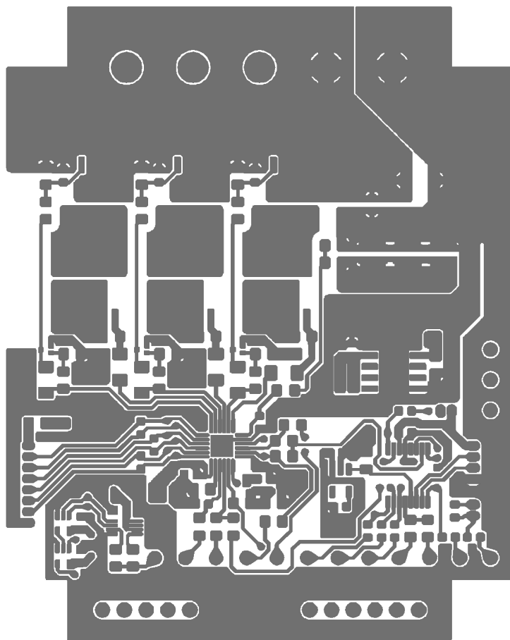
Top_Layer
