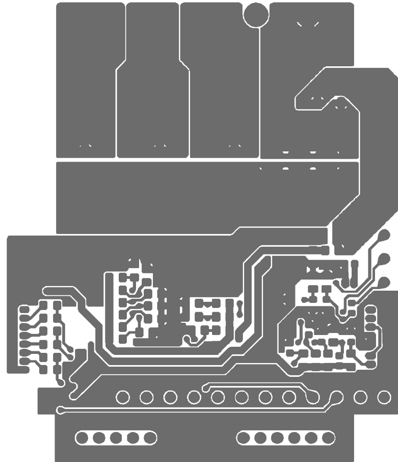
Bottom_Layer
