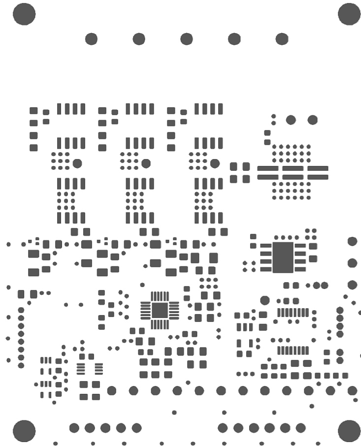
Top_Mask
