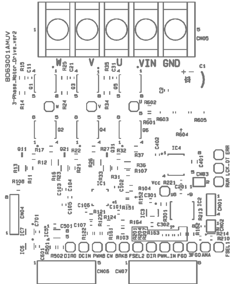
Top_Silk
