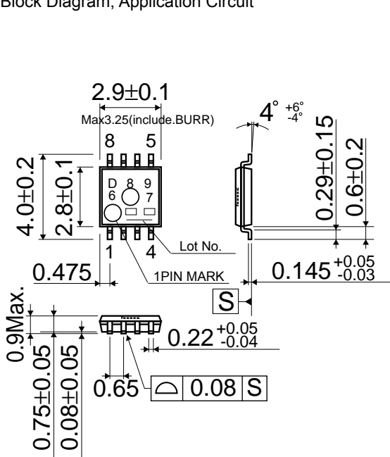
Fig.1 BD8967FVM View
