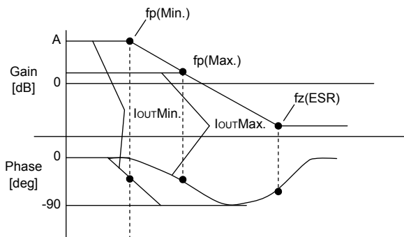
Fig.28 Open loop gain characteristics
