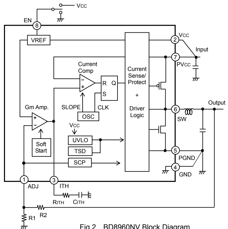
Fig.2 BD8960NV Block Diagram
