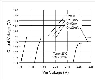
Fig. 38. Line Regulation
