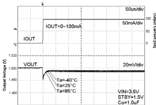
Fig. 81. Load Response
