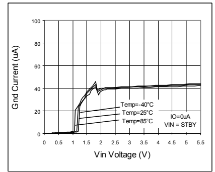
Fig. 39. Circuit Current IGND
