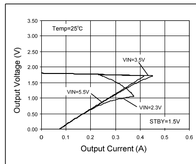
Fig. 44. OCP Threshold
