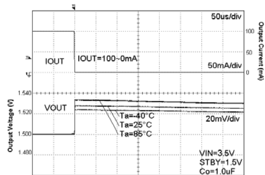
Fig. 82. Load Response
