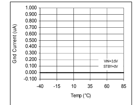
Fig. 48. IGND vs. Temp (STBY)
