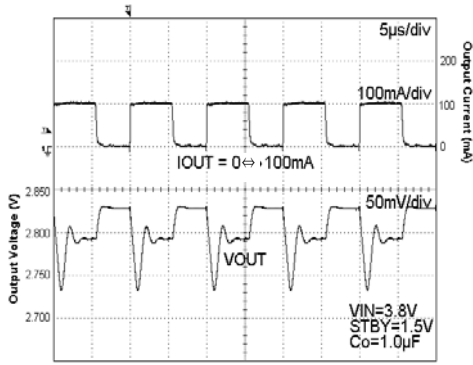
Fig. 29. Load Response Current Pulse=100kHz
