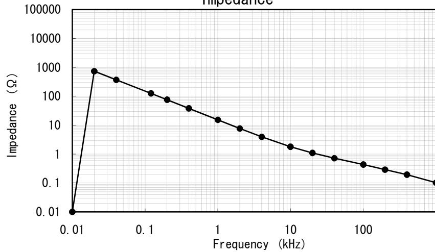
Impedance
