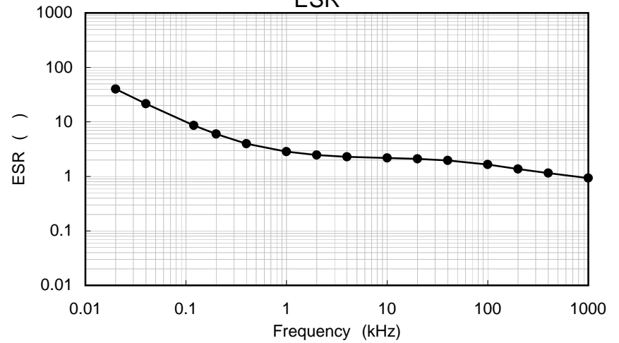
ESR ( )
