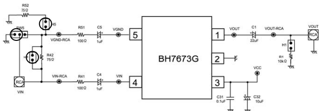
Fig.6 CMRR measurement Make SW5 connection H4 at the circuit and on the opposite side and make H5 ON.
