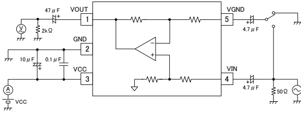
Fig.1 Test Circuit Diagram Test circuit diagrams are used for shipment inspections, and differ from application circuits.
