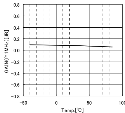
Fig.14 Gain vs. Ambient Temperature
