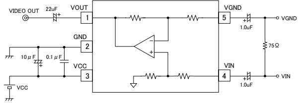
Fig.2 Application circuit examples See pages 6 for description of how to determine the capacity of I/O coupling capacitors.
