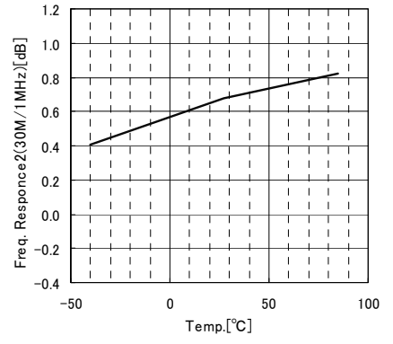
Fig. 18 Frequency Response2 vs. Ambient Temperature
