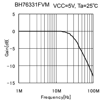
Fig.40 Frequency Response
