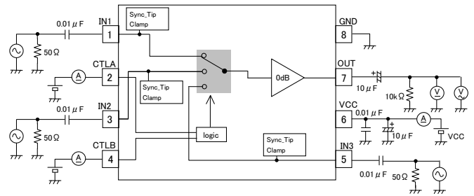
Fig. 6 BH76332FVM/BH76333FVM Test Circuit Diagram
