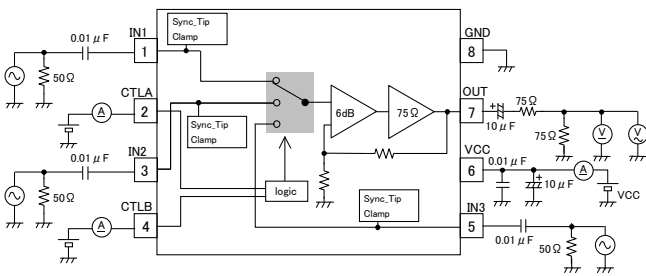
Fig. 5 BH76330FVM/BH76331FVM Test Circuit Diagram
