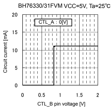
Fig.45 CTLb pin voltage vs Circuit Current (CLT threshold)
