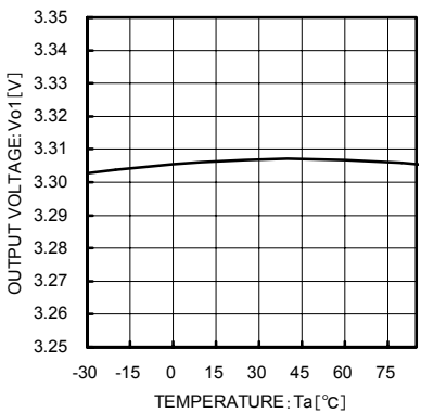
Fig.10 Output Voltage vs Temperature (3.3 V output)
