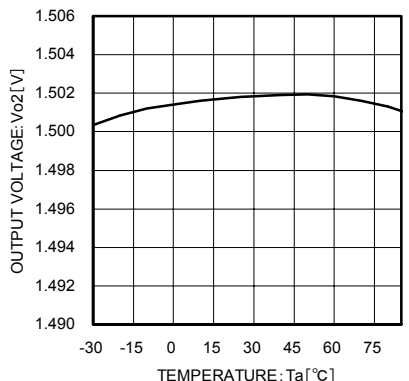
Fig.11 Output Voltage vs Temperature (Variable output: 1.5 V)
