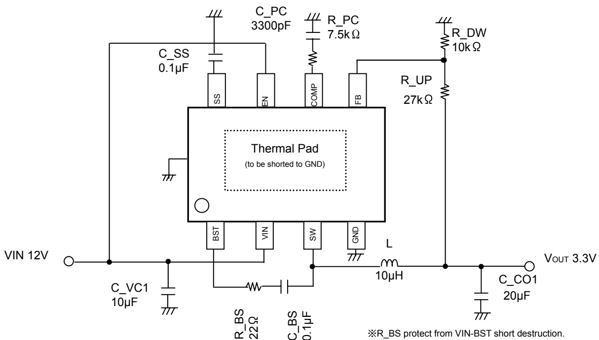
Fig.1 Typical Application Circuit
