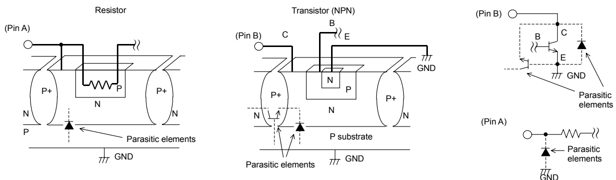
Fig.29 Example of a Simple Monolithic IC Architecture
