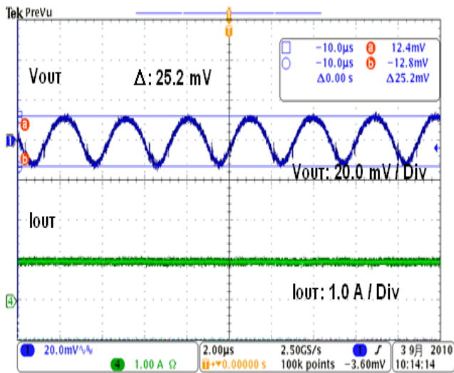
Fig.14 Output Ripple Voltage (VIN= 12V VOUT= 3.3V L= 10μH Cout =20μF I out= 1.0A )
