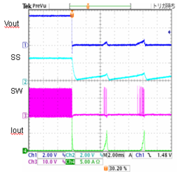
Fig.11 OverCurrent Protection
