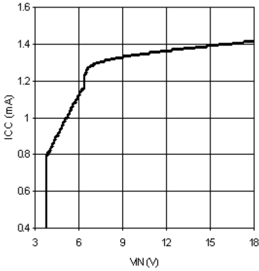
Fig.4 Circuit Current (No switching)
