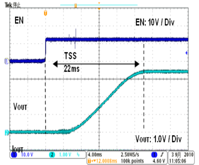
Fig.17 Start Up waveform (VIN= 12V VOUT= 3.3V L= 10 \mu\text{H} CSS= 0.1 \mu\text{F} )
