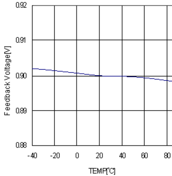
Fig.7 Feedback voltage
