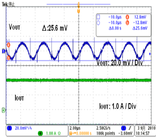
Fig.16 Output Ripple Voltage (VIN= 12V VOUT= 3.3V L= 10 \mu\text{H} Cout =20 \mu\text{F} I out= 2.0A)
