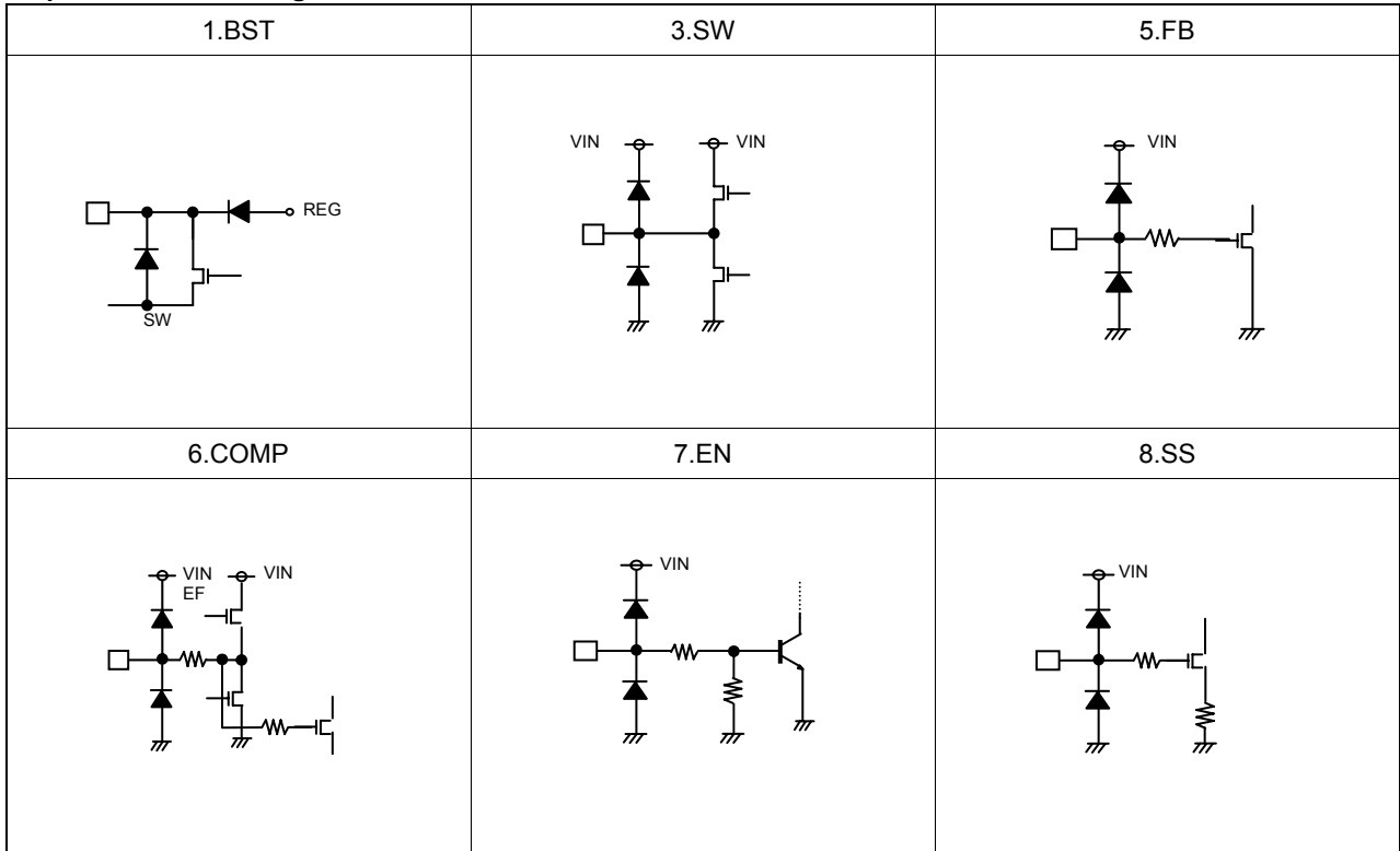
Fig.28 I/O Equivalent Circuit
