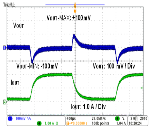
Fig.15 Transient Response (VIN= 12V VOUT= 3.3V L= 10μH Cout =20μF Iout= 0.2-2.0A)
