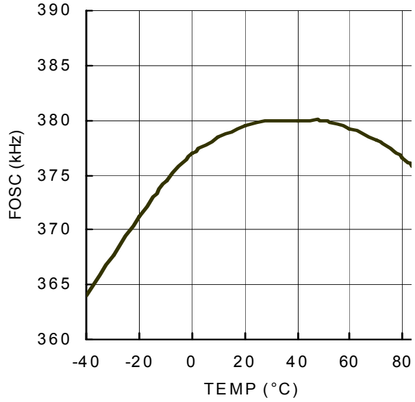
Fig.9 Operating Frequency
