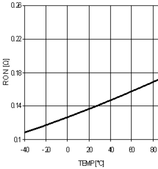
Fig.8 Hi, Low-Side On-resistance
