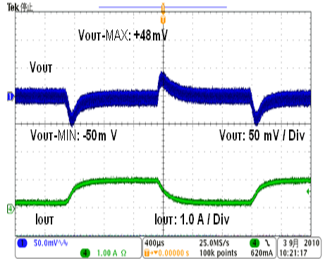
Fig.13 Transient Response (VIN= 12V VOUT= 3.3V L= 10μH Cout =20μF Iout= 0.2-1.0A )
