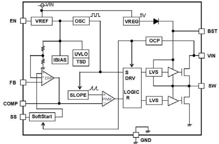
Fig. 3 Block Diagram
