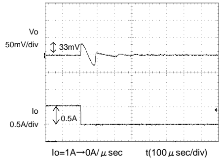
Fig.6 Transient Response (0.5→0A) Co=22 \mu F, Cfb=1000pF
