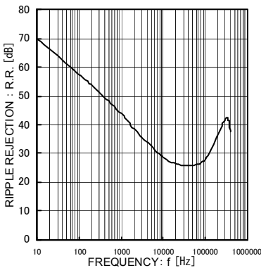
Fig.19 Ripple Rejection (Io=100mA)
