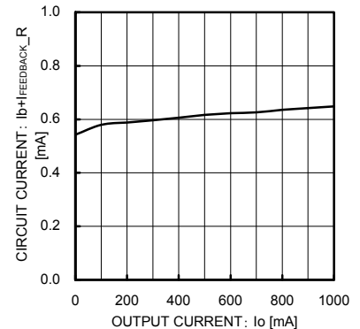
Fig.21 Circuit Current (Io=0mA→1000 mA)
