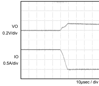
Fig.2 Transient Response(1.0→0A) Co=2.2µF
