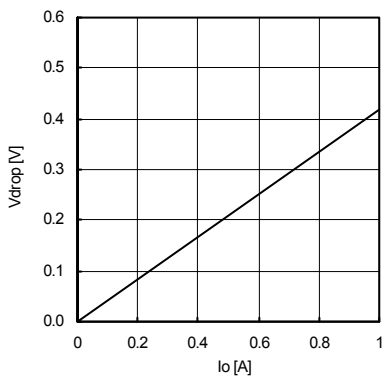
Fig.34 Minimum dropout Voltage3 (VCC=3.3V)
