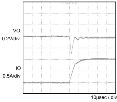
Fig.1 Transient Response(0→1.0A) Co=2.2µF
