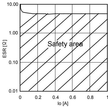
Fig.29 ESR-IO characteristics (Co=2.2µF)
