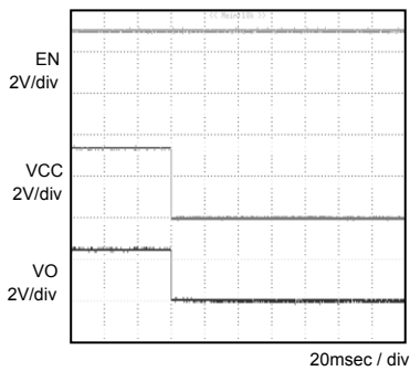
Fig.4 OFF sequence 1 Co=2.2µF
