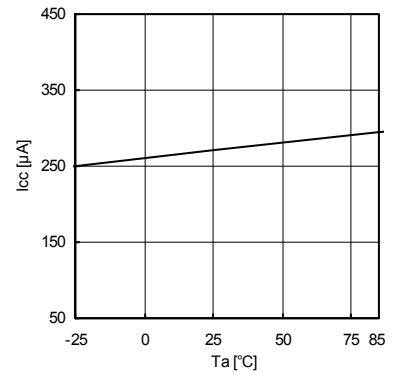
Fig.9 Ta-ICC
