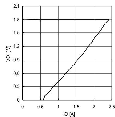
Fig.22 OCP (VCC=5V, VO=1.8V)
