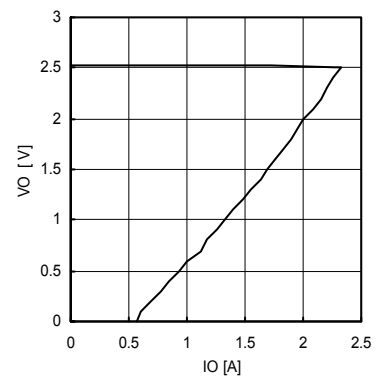
Fig.21 OCP (VCC=5V, VO=2.5V)
