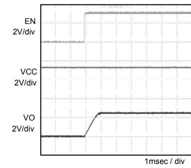
Fig.5 Input sequence2 Co=2.2µF
