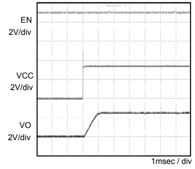
Fig.3 Input sequence1 Co=2.2µF
