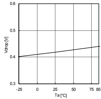
Fig.32 Minimum dropout Voltage 1 (VCC=3.3V, IO=1.0A)
