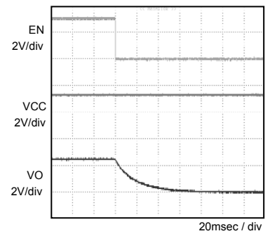
Fig.6 OFF sequence 2 Co=2.2µF
