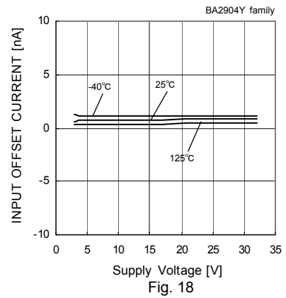
Fig. 18 Input Offset Current – Supply Voltage ( V_{icm}=0[V] , V_{OUT}=1.4[V] )
