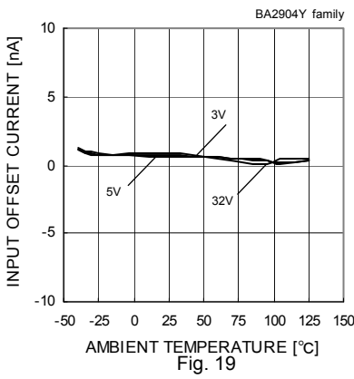
Fig. 19 Input Offset Current – Ambient Temperature ( V_{icm}=0[V] , V_{OUT}=1.4[V] )
