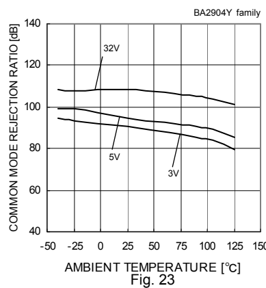
Fig. 23 Common Mode Rejection Ratio – Ambient Temperature
