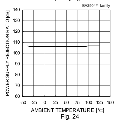
Fig. 24 Power Supply Rejection Ratio – Ambient Temperature
