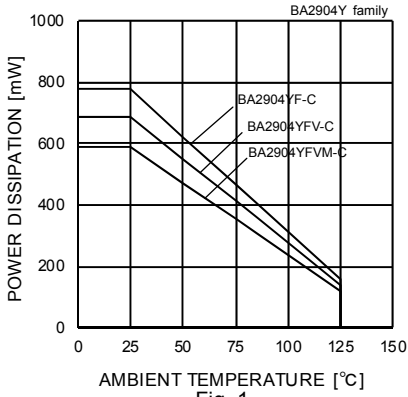
Fig. 1 Derating Curve
