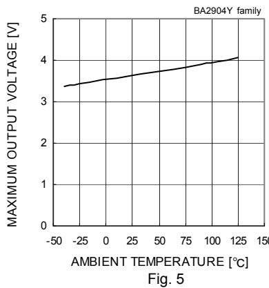
Fig. 5 Maximum Output Voltage - Ambient Temperature (VCC=5[V], RL=2[kΩ])
