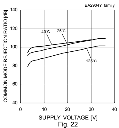
Fig. 22 Common Mode Rejection Ratio – Supply Voltage
