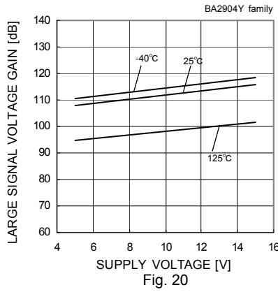
Fig. 20 Large Signal Voltage Gain – Supply Voltage( R_L=2[k\Omega] )
