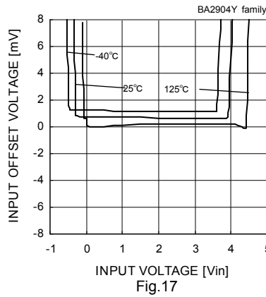
Fig. 17 Input Offset Voltage – Input Voltage ( V_{CC}=5[V] )
