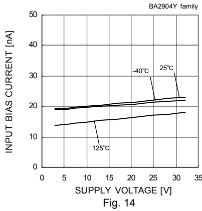
Fig. 14 Input Bias Current – Supply Voltage ( V_{icm}=0[V] , V_{OUT}=1.4[V] )
