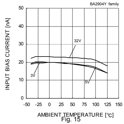
Fig. 15 Input Bias Current – Ambient Temperature ( V_{icm}=0[V] , V_{OUT}=1.4[V] )
