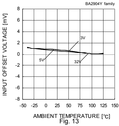
Fig. 13 Input Offset Voltage – Ambient Temperature ( V_{icm}=0[V] , V_{OUT}=1.4[V] )
