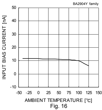
Fig. 16 Input Bias Current – Ambient Temperature ( V_{CC}=30[V] , V_{icm}=28[V] , V_{OUT}=1.4[V] )
