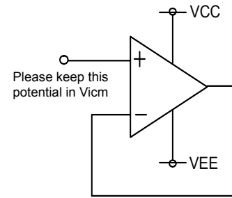
Fig. 56 Example of processing unused circuit
