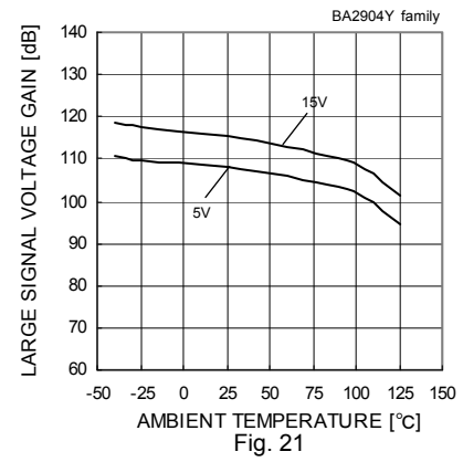
Fig. 21 Large Signal Voltage Gain – Ambient Temperature ( R_L=2[k\Omega] )
