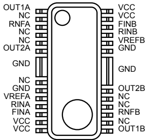
Fig.8 HSOP25(TOP VIEW)
