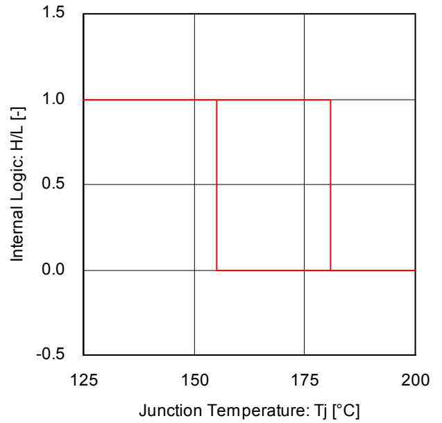
Fig.22 Thermal shutdown
