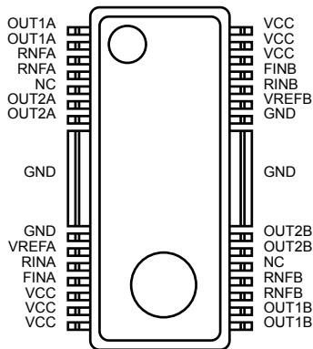
Fig.12 HSOP-M28(TOP VIEW)
