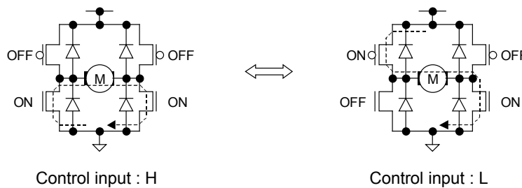
Fig.40 PWM control mode B operation (output stage)
