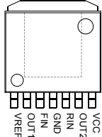
Fig.4 HRP7(TOP VIEW)
