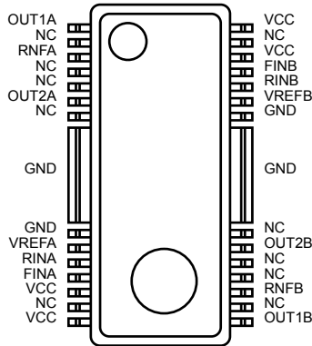
Fig.10 HSOP-M28(TOP VIEW)
