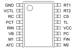
Fig.16 BA6951FS (SSOP-A16)
