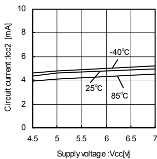
Fig.1 Circuit Current 2
