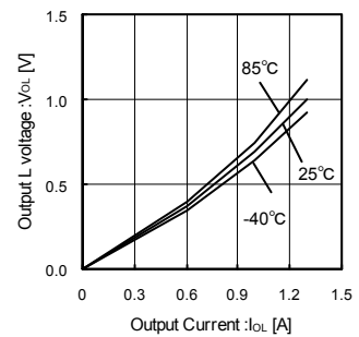
Fig.3 Output Saturation Voltage at Low Level
