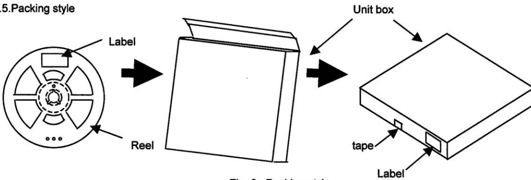
Fig. 6 Packing style
