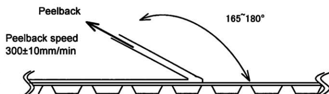
Fig. 8 Test method
