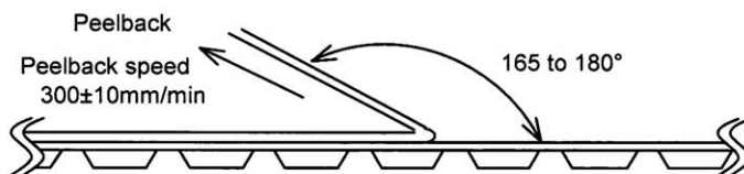
Fig. 8 Test method
