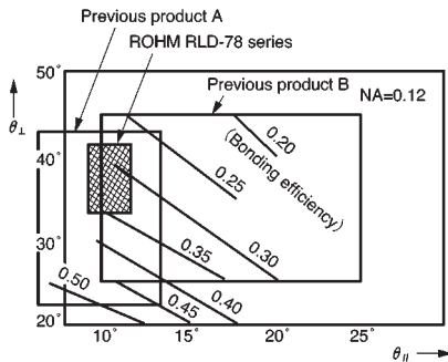
Fig. 9 Far-field dispersion
