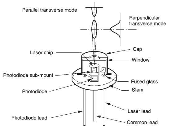
Fig. 8 Structure of complete small \phi 5.6 mm laser diode device
