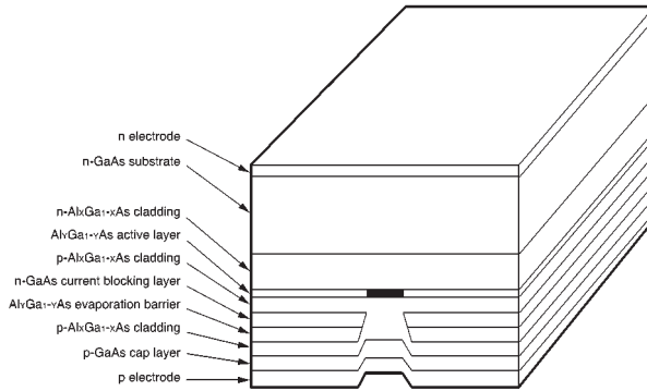
Fig. 6 Laser chip structure
