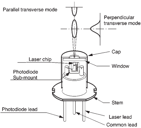
Fig. 7 Structure of complete ultra-small \phi 3.3 mm laser diode device
