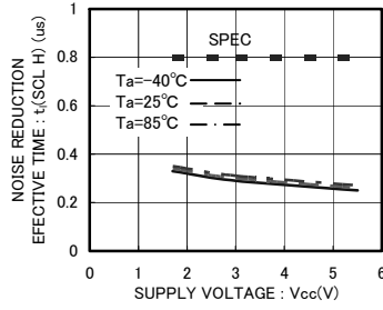
Fig.26 Noise reduction effective time t_1(\text{SCL H})
