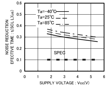
Fig.27 Noise reduction effective time t_1(\text{SCL L})
