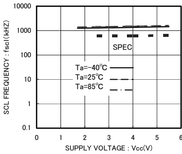
Fig.13 SCL frequency f_{SCL}
