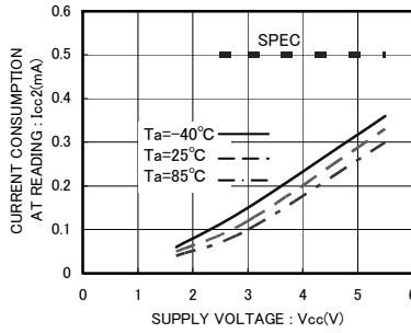
Fig.11 Current consumption at READ operation I_{cc2} (fsci=400kHz)
