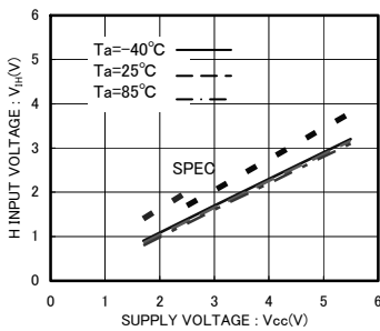
Fig.4 'H' input voltage V_{IH} (A0,A1,A2,SCL,SDA,WP)
