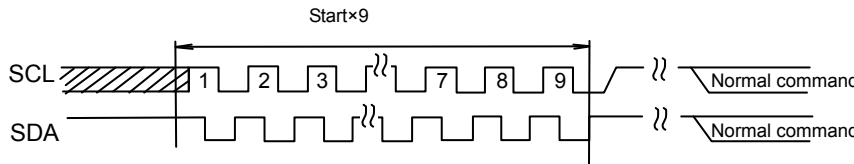
Fig.39-(c) START x 9 + command input
