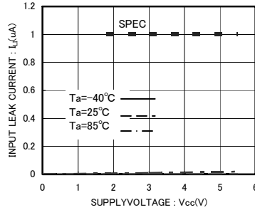
Fig.8 Input leak current I_I (A0,A1,A2,SCL,WP)
