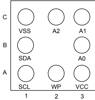
Fig.3 BU9880GUL-W(bottom view)
