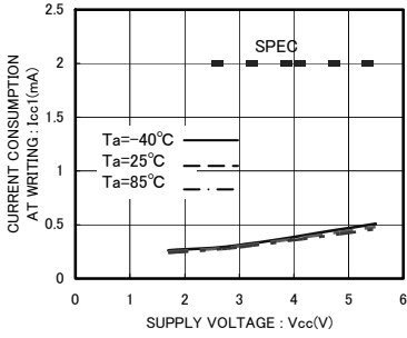
Fig.10 Current consumption at WRITE operation I_{cc1} (fsci=400kHz)
