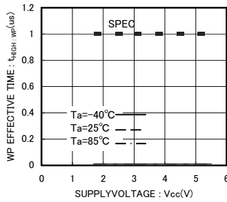
Fig.31 WP effective time t_{HIGH:WP}
