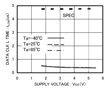
Fig.15 Data clock Low Period t_{LOW}
