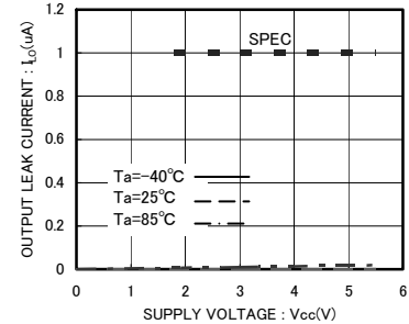
Fig.9 Output leak current I_{LO}(SDA)
