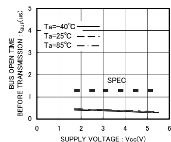
Fig.24 BUS open time before transmission t_{BUF}
