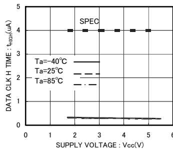
Fig.14 Data clock High Period t_{HIGH}
