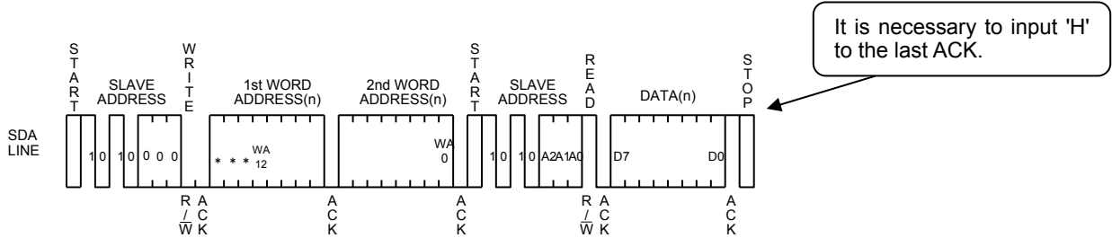
Fig.36 Random read cycle
