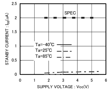
Fig.12 Standby operation I_{sb}
