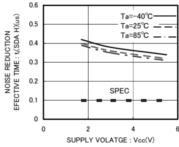
Fig.28 Noise reduction effective time t_1(\text{SDA H})
