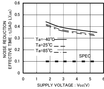
Fig.29 Noise reduction effective time t_1(\text{SDA L})
