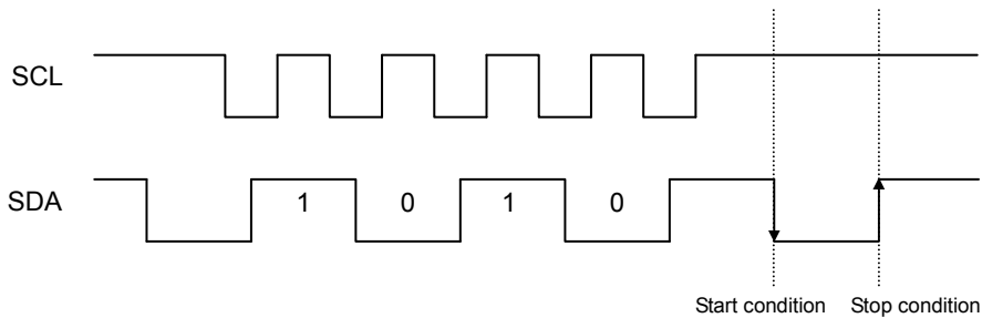
Fig.42 Case of cancel by start, stop condition during slave address input
