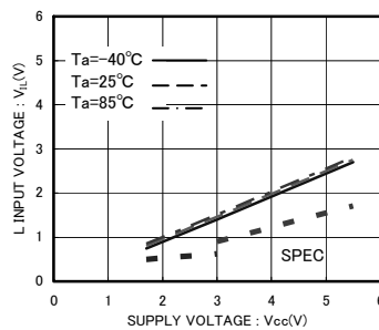
Fig.5 'L' input voltage V_{IL} (A0,A1,A2,SCL,SDA,WP)
