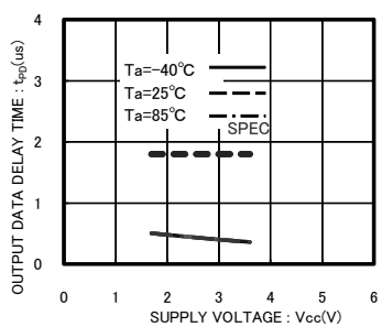
Fig.19 'L' Data output delay time t_{PO0}
