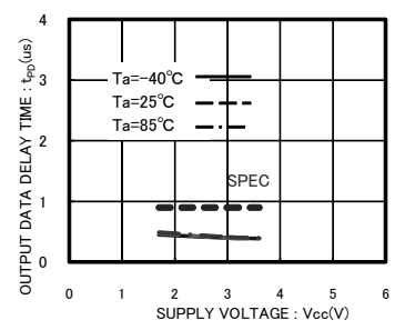
Fig.20 'H' Data output delay time t_{PO1}
