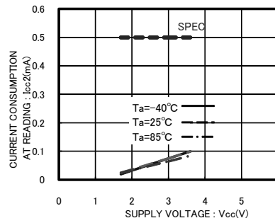
Fig.10 Current consumption at READ operation I_{CC2} (fsc1=400kHz)
