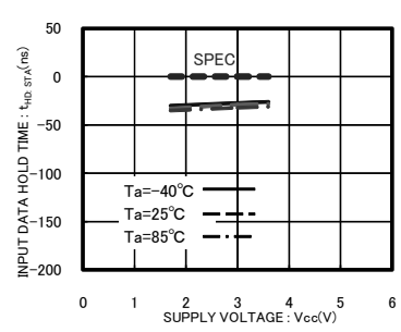
Fig.17 Input Data Hold Time t_{HD:DAT(HIGH)}
