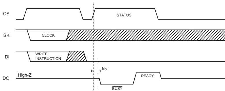
Fig. 49 R/\overline{B} status output timing chart
