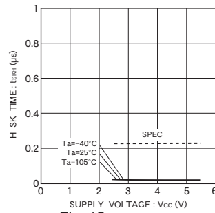
Fig. 15 SK high time t_{sKH}
