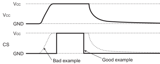
Fig. 56 Timing at power ON/OFF
