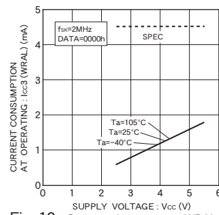
Fig. 12 Consumption current at WRAL action I_{CC3} (WRAL, f_{sk}=2\text{MHz} )
