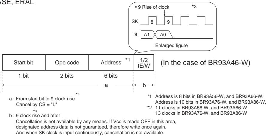
Fig. 38 ERASE, ERAL cancel available timing
