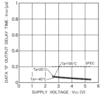
Fig. 22 Data "0" output delay time t_{po0}
