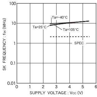
Fig. 14 SK frequency f_{sk}
