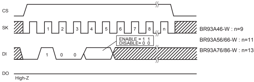
Fig. 33 Write enable (WEN) / disable (WDS) cycle
