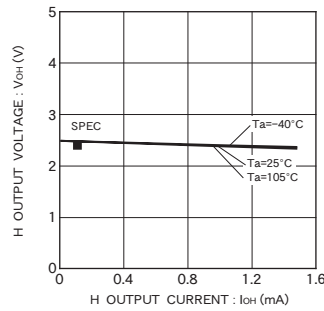
Fig. 6 H output voltage V_{OH-I_{OH}} ( V_{CC}=2.5\text{V} )
