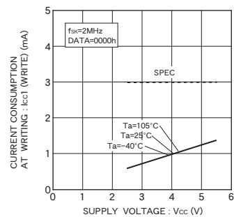
Fig. 10 Current consumption at WRITE action I_{CC1} (WRITE, f_{sk}=2\text{MHz} )
