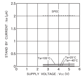
Fig. 13 Consumption current at standby action I_{SB}
