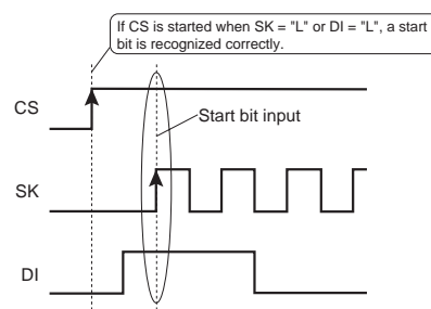
Fig. 40 Normal action timing
