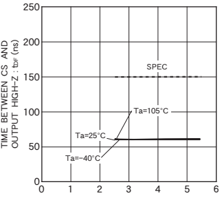
Fig. 25 Time from CS to High-Z t_{df}
