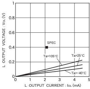
Fig. 5 L output voltage V_{OL-I_{OL}} ( V_{CC}=4.0\text{V} )
