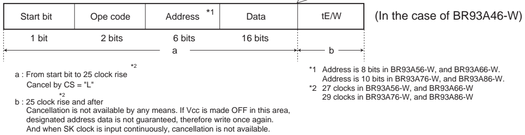
Fig. 37 WRITE, WRAL cancel available timing
