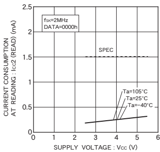
Fig. 11 Consumption current at READ action I_{CC2} (READ, f_{sk}=2\text{MHz} )
