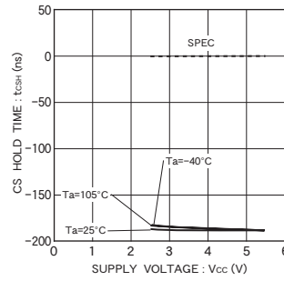
Fig. 18 CS hold time t_{cSH}
