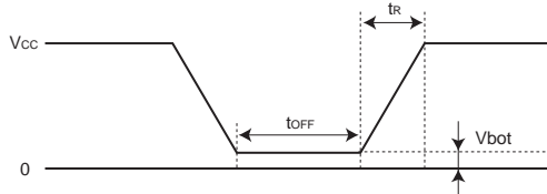
Fig. 57 Rise waveform diagram
