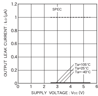
Fig. 9 Output leak current I_{LO} (DO)
