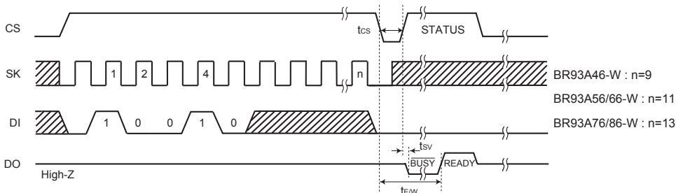
Fig. 35 Chip erase cycle timing
