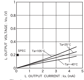
Fig. 4 L output voltage V_{OL-I_{OL}} ( V_{CC}=2.5\text{V} )
