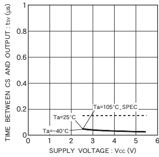
Fig. 24 Time from CS to output establishment t_{sv}
