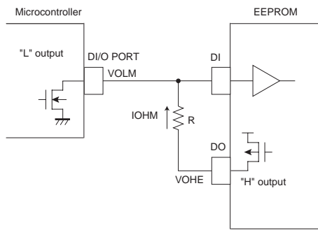
Fig. 55 Circuit at DI, DO direct connection (Microcontroller DI/O "L" output, EEPROM "H" output)
