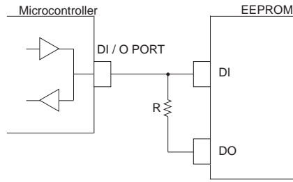
Fig. 50 DI, DO control line common connection
