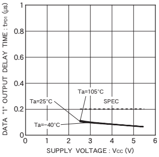
Fig. 23 Output data "1" delay time t_{pd1}
