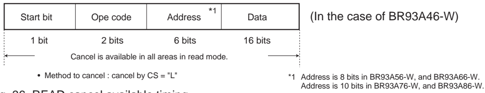
Fig. 36 READ cancel available timing
