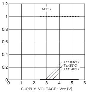
Fig. 8 Input leak current I_L (CS,SK,DI)
