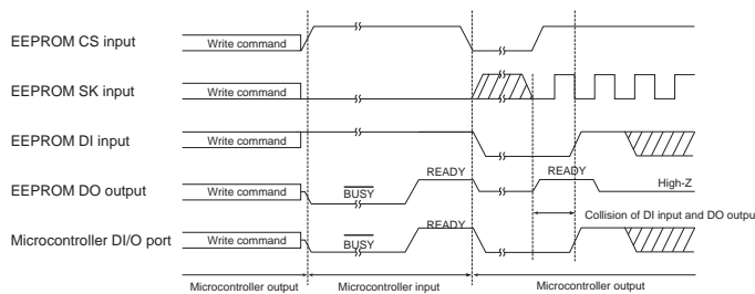
Fig. 52 Collision timing at DI, DO direct connection
