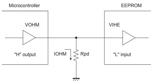
Fig. 45 CS pull down resistance
