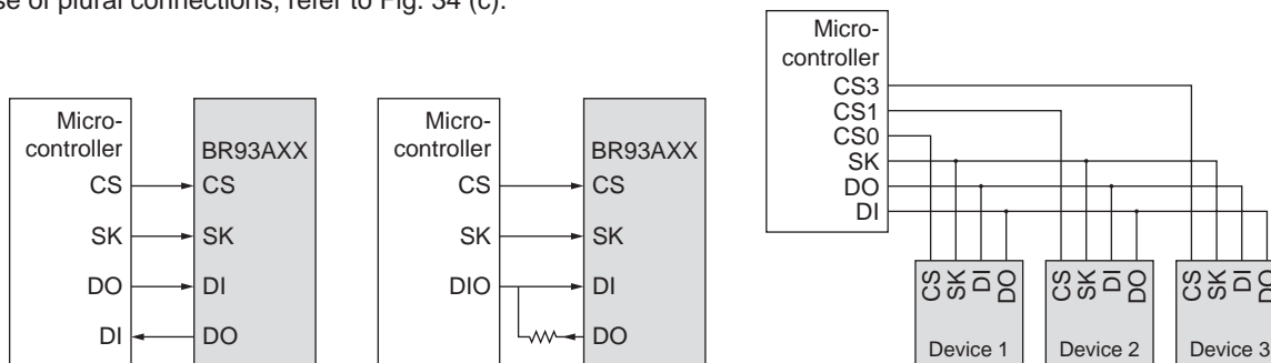
Fig. 29-(a) Connection by 4 lines Fig. 29-(b) Connection by 3 lines Fig. 29-(c) Connection example of plural devices
