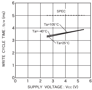
Fig. 26 Write cycle time t_{eW}
