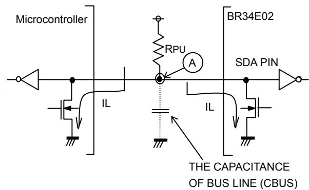
Fig.43 I/O Circuit
