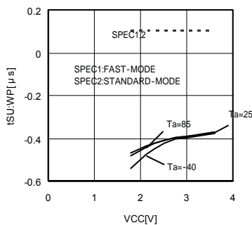
Fig.31 WP Setup Time t_{SU:WP}
