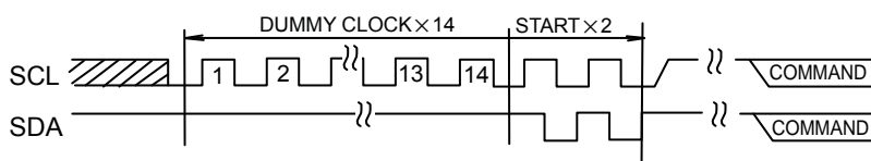
Fig.39-(a) DUMMY CLOCK \times 14 + START \times 2
