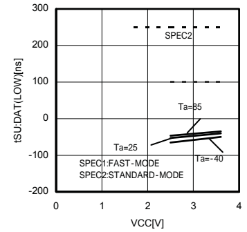
Fig.21 Input Data Setup Time tSU:DAT(LOW)
