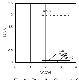
Fig.12 Standby Current ISB
