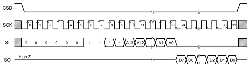
Fig.34 Read command
