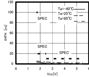
Fig.25 HOLDB setting hold time tHFH
