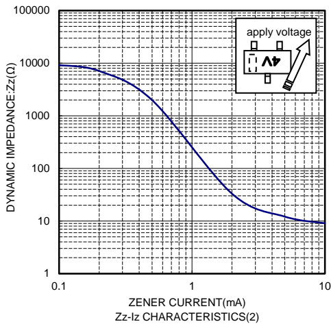
Zz-Iz CHARACTERISTICS(2)
