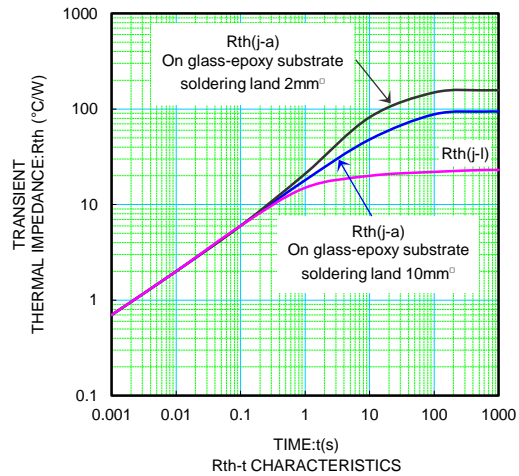
R_{th} \cdot t CHARACTERISTICS
