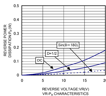
VR-Pr CHARACTERISTICS
