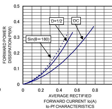
Io-PF CHARACTERISTICS
