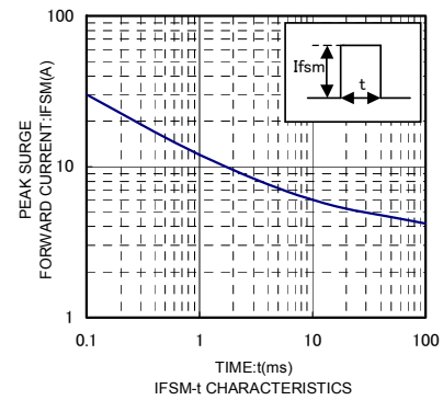
IFSM-t CHARACTERISTICS
