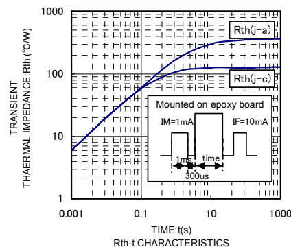
Rth-t CHARACTERISTICS
