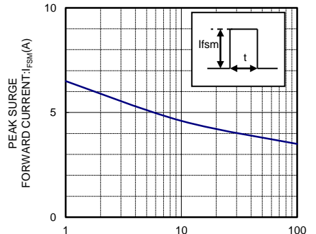
I_{FSM} - t CHARACTERISTICS
