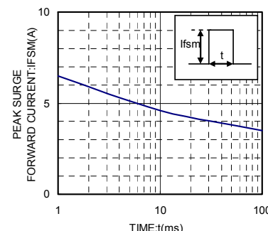
IFSM-t CHARACTERISTICS
