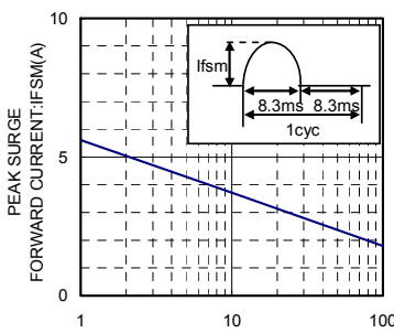
IFSM-CYCLE CHARACTERISTICS
