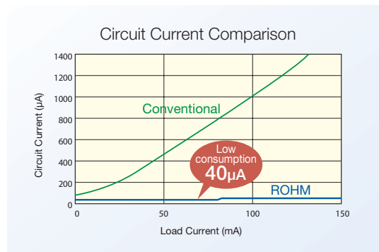
Figure 1. The P-channel MOSFET at the output stage of ROHM's line of Standard CMOS LDOs results in a dramatically lower circuit current than possible with convention bipolar types.
