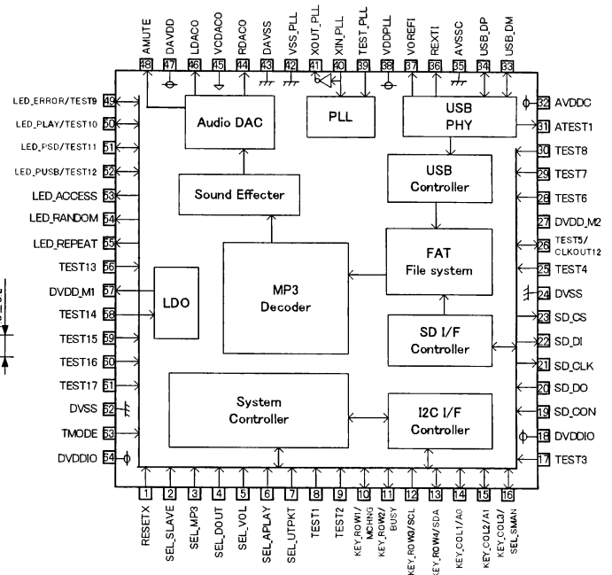
Figure 2. Block diagram
