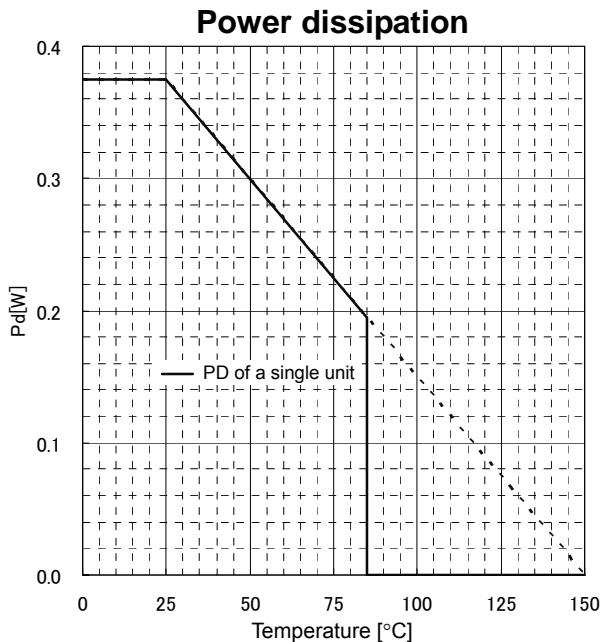
Fig. 1 BD8919F Power Dissipation
