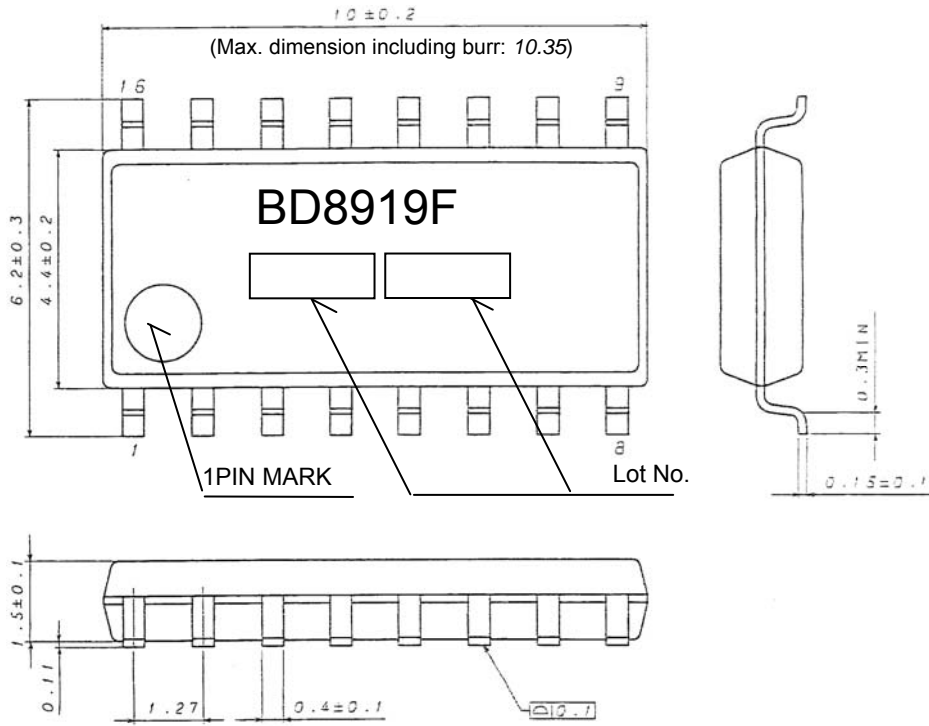
Fig. 3 SOP16 Package Dimension
